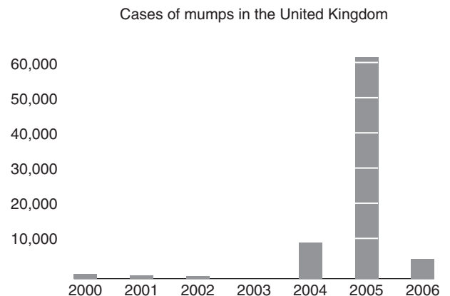
FIGURE 17.3 In 2005, there were more than 63,500 cases of Mumps in the United Kingdom (WHO, 2007b) (Adapted from Myers and Pineda (2008) with permission of the publisher.)
