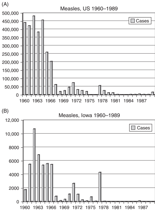
FIGURE 17.1 Measles in (A) the United States (Centers for Disease Control and Prevention, 1995) and (B) Iowa (Iowa Department of Health, 2007, www.idph.state.ia.us/adper/pdf/cade/decades/pdf ) 1960–1989. Measles vaccine was licensed in 1963. Mandatory immunization laws were enacted widely by states in the late 1960s and 1970s. Iowa enacted its immunization law in 1977 (Iowa Administrative Code, 1977).
